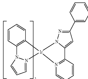
\lambda_{\text{max}} 485 nm (DCM)
