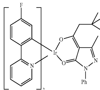
\lambda_{\text{max}} 493 nm (DCM)
